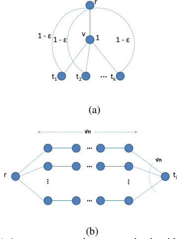
Figure 1. (a) A counter-example to a greedy algorithm for the online node-weighted Steiner tree problem. All the curved edges have cost 1 - \epsilon and the straight edges have cost 0. Vertex v has cost 1; all other vertices are terminals and have cost 0. In this example, the vertices r, t_1, t_2, \dots, t_k appear as terminals. Since each terminal has a private path of cost 1 - \epsilon to r , the greedy algorithm selects these private paths with total cost (1 - \epsilon)k , whereas the optimal solution chooses the paths through vertex v and has cost 1. Choosing \epsilon to be an arbitrarily small positive constant leads to a lower bound of k on the competitive ratio of this algorithm. (b) An example exhibiting the difficulty of online rounding of the natural LP relaxation of NW Steiner tree. If each edge and vertex has a value of 1/\sqrt{n} in the fractional solution, then an independent rounding of the edges and vertices does not produce a feasible solution. On the other hand, since the value on an edge or vertex accumulates over multiple rounds, dependent rounding may produce an integer solution that is polynomially more expensive than the fractional solution.
